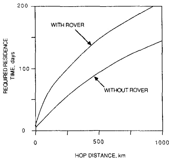
Fig. 5. Residence time required for propellant production as a function of hop distance
